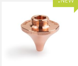
Bevel Cut Nozzle M12 Nozzle EAR
