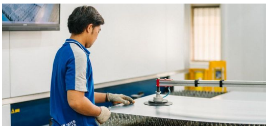
<p>The solar panel mounting bracket consists of around 100 individual parts. They are precisely cut and perforated on a TruLaser 3060 fiber 6 kW laser cutting system and a TruLaser 3030 fiber with 24 kW from TRUMPF.</p>
